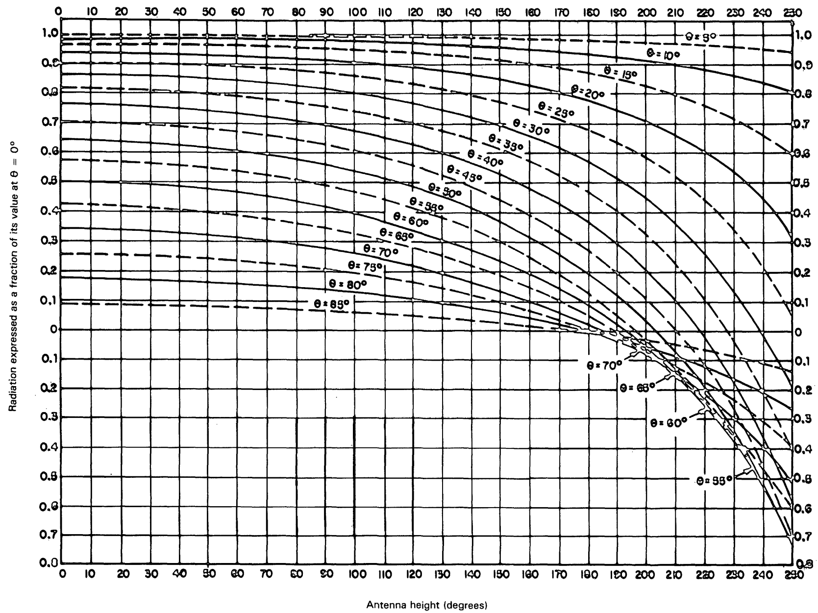
FIGURE 2.7 - Vertical plane radiation of simple vertical antennas as a function of electrical tower height for various values of elevation angle ( \theta ) (provided for information purposes)
