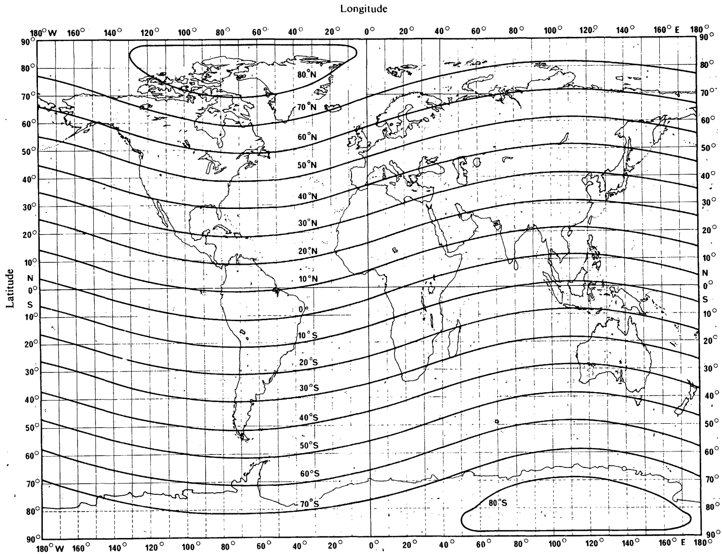
FIGURE 2 Geomagnetic latitudes
