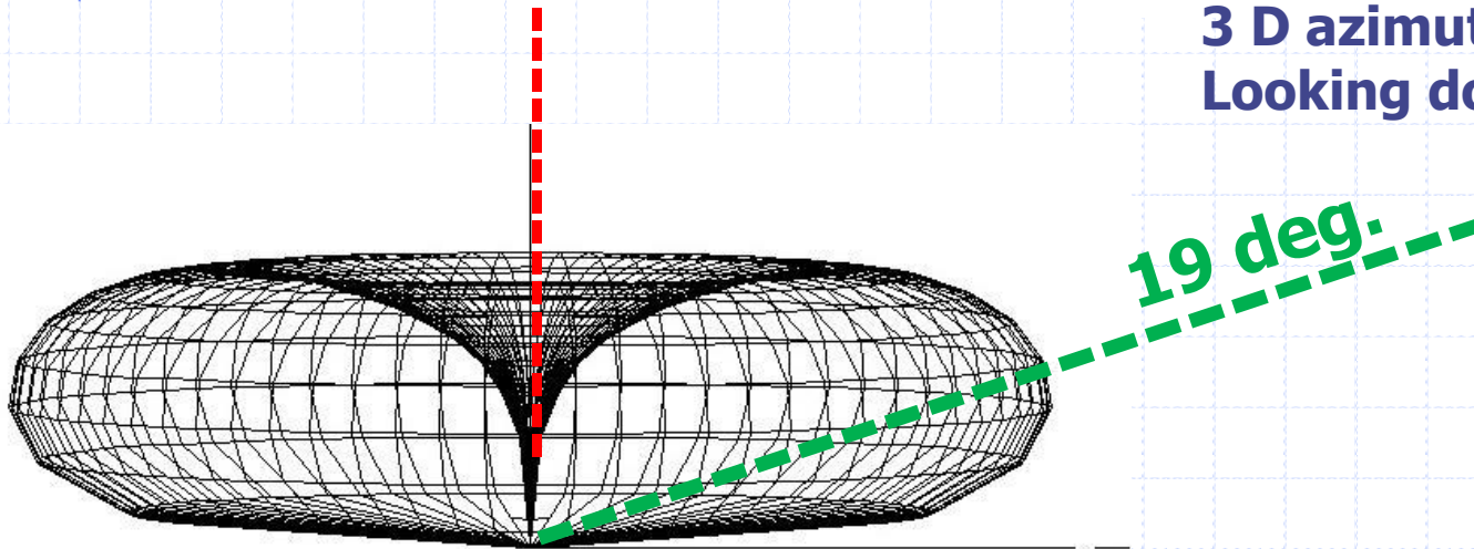
Side view of antenna – 3D elevation plot
