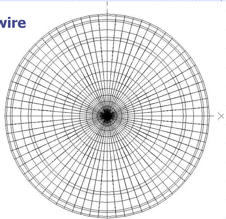
3 D azimuth plot of antenna Looking down from the top
