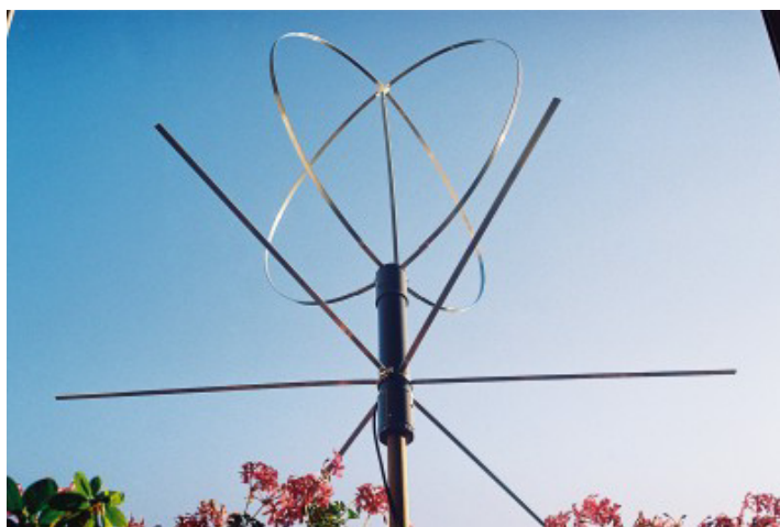
Fig 6 ' VHF Eggbeater '
