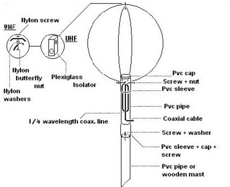
Fig 4 Practical building
