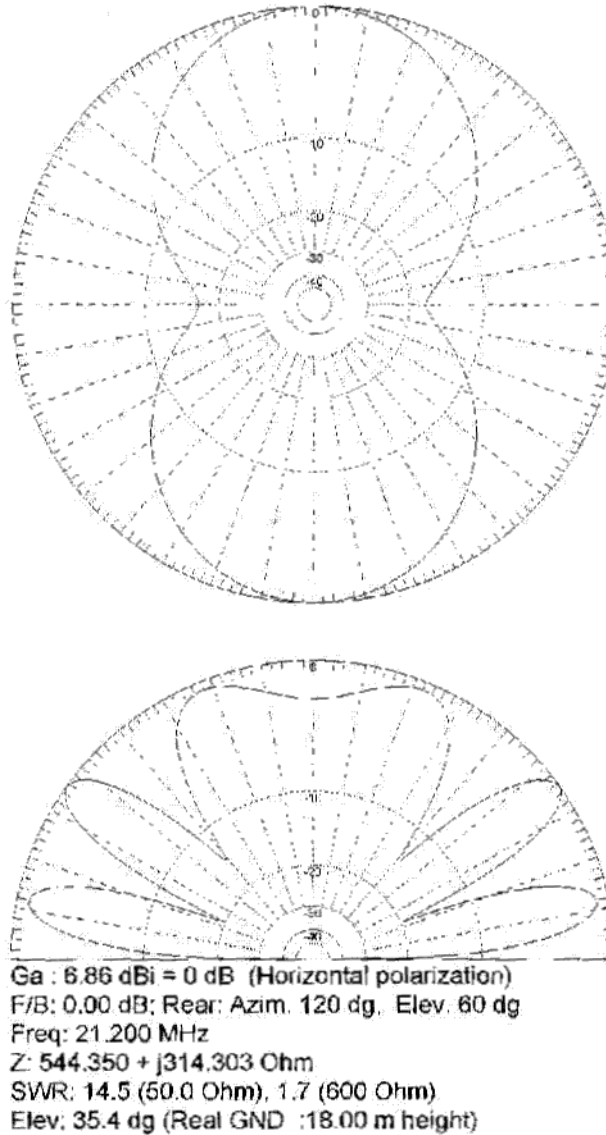
Figure 14.4: Radiation Pattern of a 30-meter Delta Loop on 15 Meters
