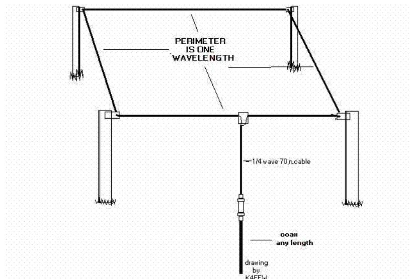
Figure 14.1: One Wavelength Horizontal Loop
