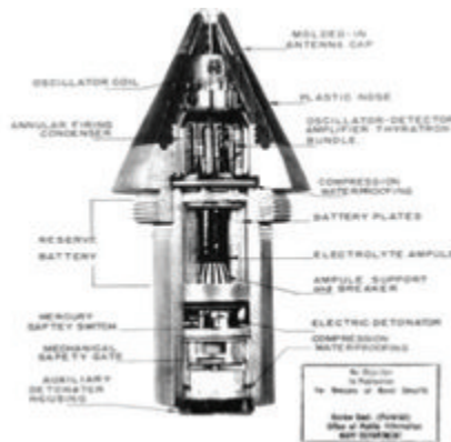
A cutaway view of a Variable Time Fuze
