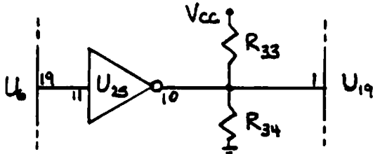
Figure 1. Revised CWID facility for the TAPR TNC.
