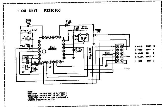
FTS-17A Circuit Diagram
