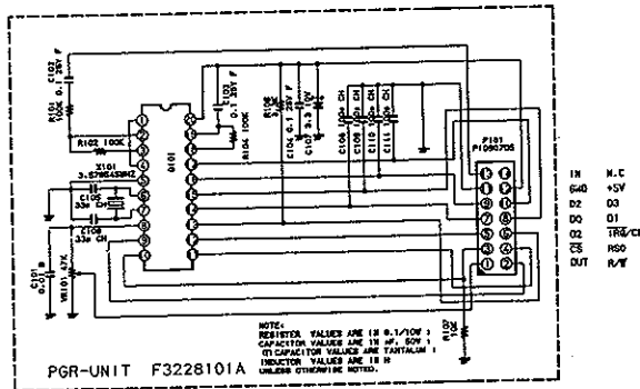
FRC-6 Circuit Diagram
