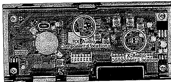
Fig. 1 Modification Component Locations
