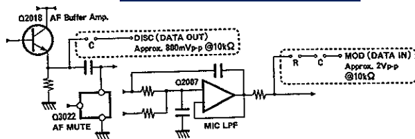
TNC DATA IN/OUT Lead Connection
