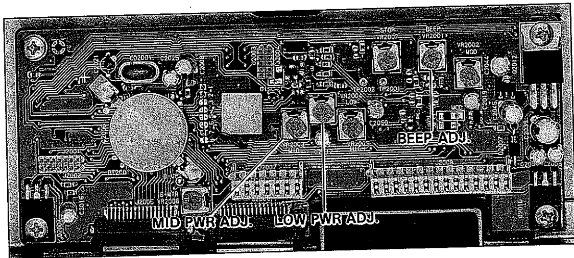
FT-2500M Internal Adjustment Locations
