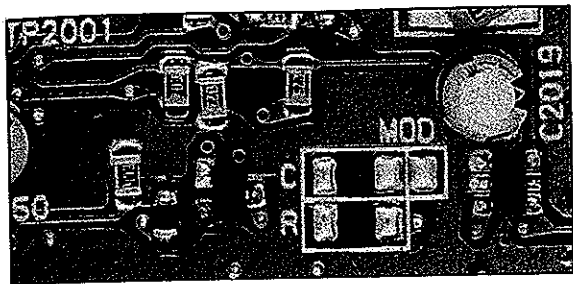
Fig. 3 TX Audio Component Location
