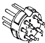
BAND DATA PLUG PINOUT
