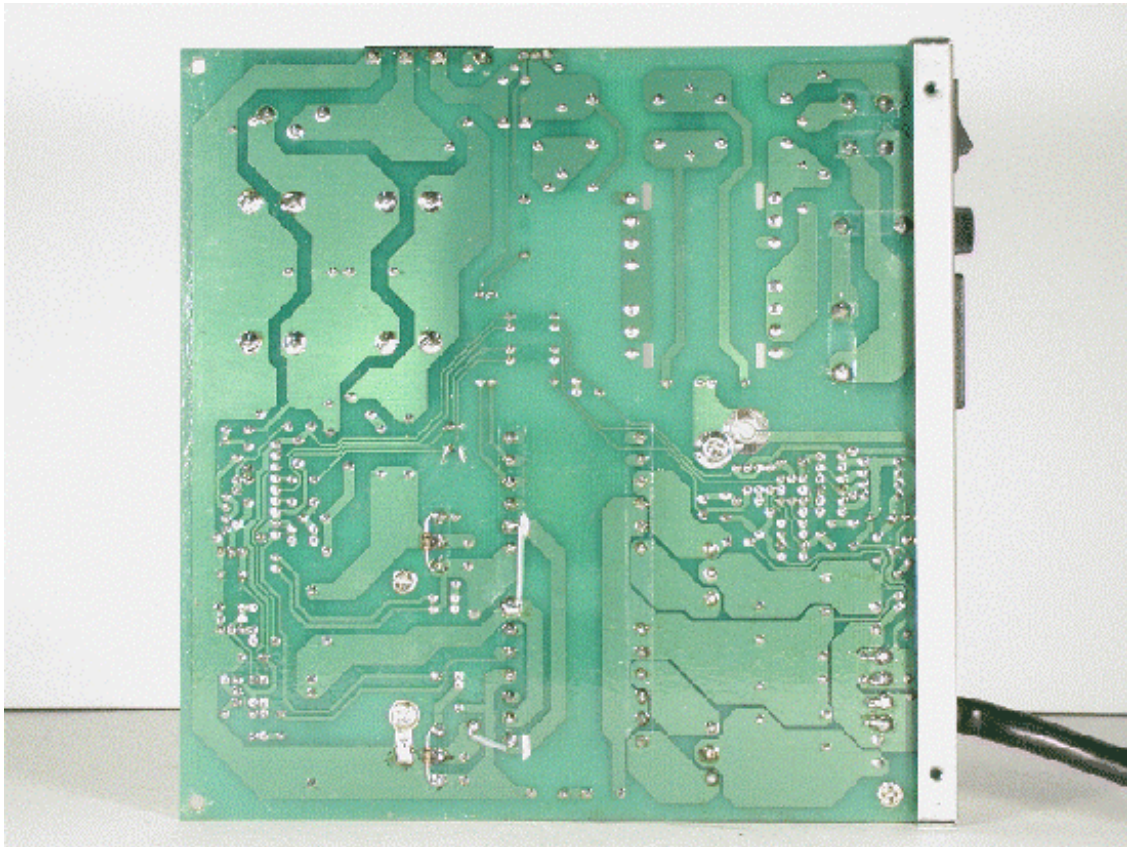
Bottom of DC Power Supply
