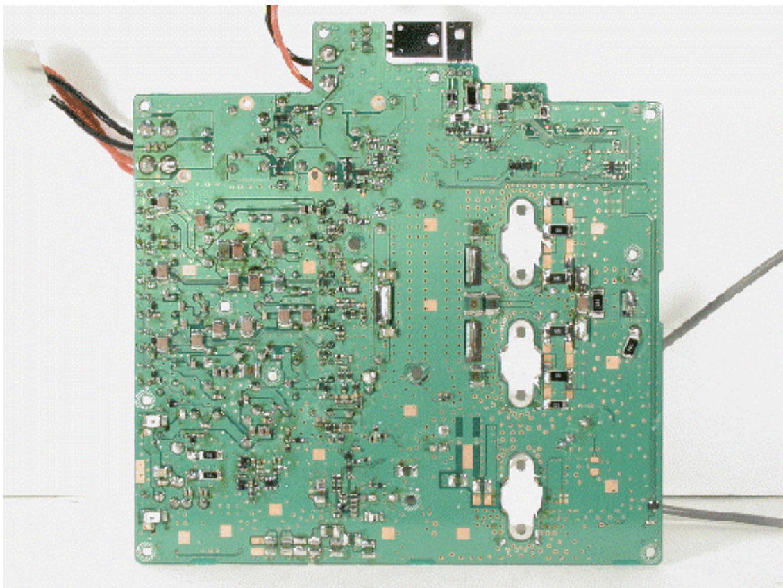
Side-B of PA-UNIT
