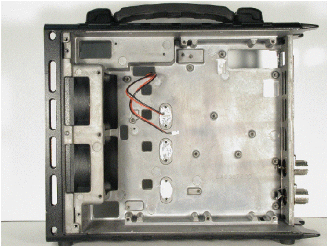
Inside Bottom of Chassis
