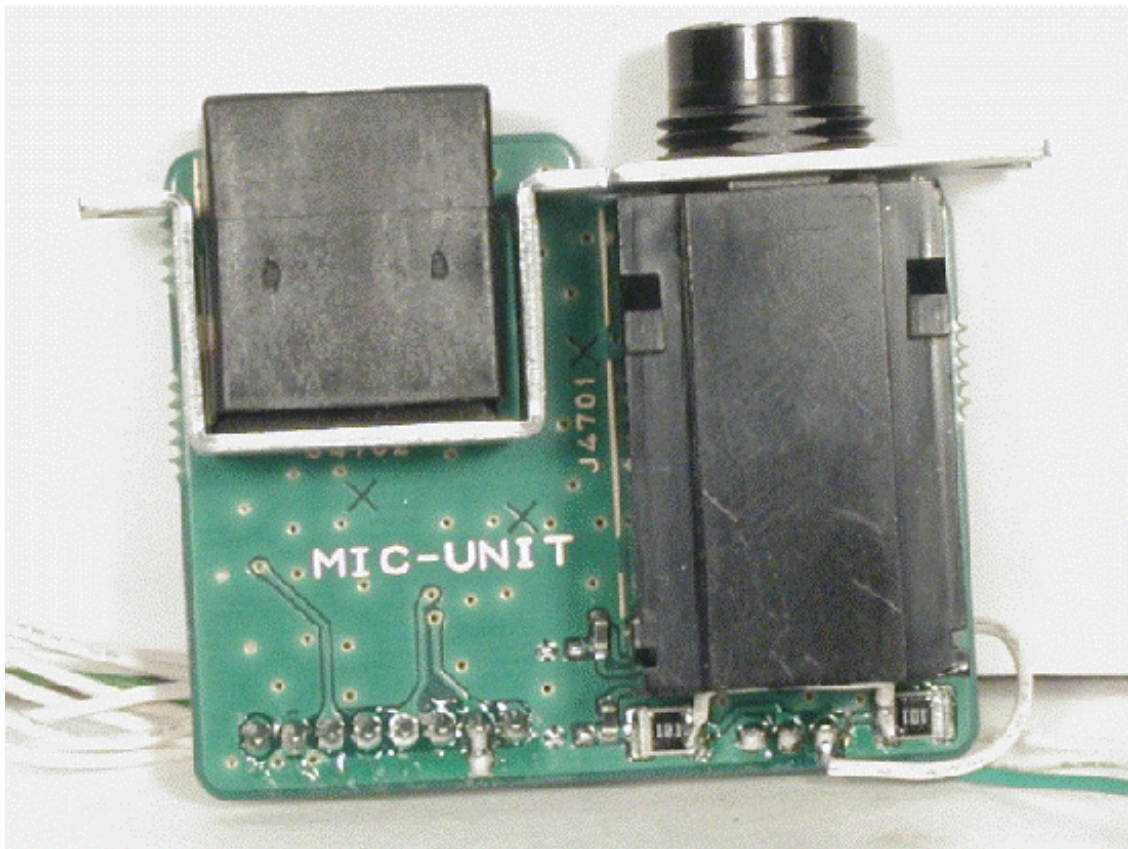
Side-A of MIC-UNIT
