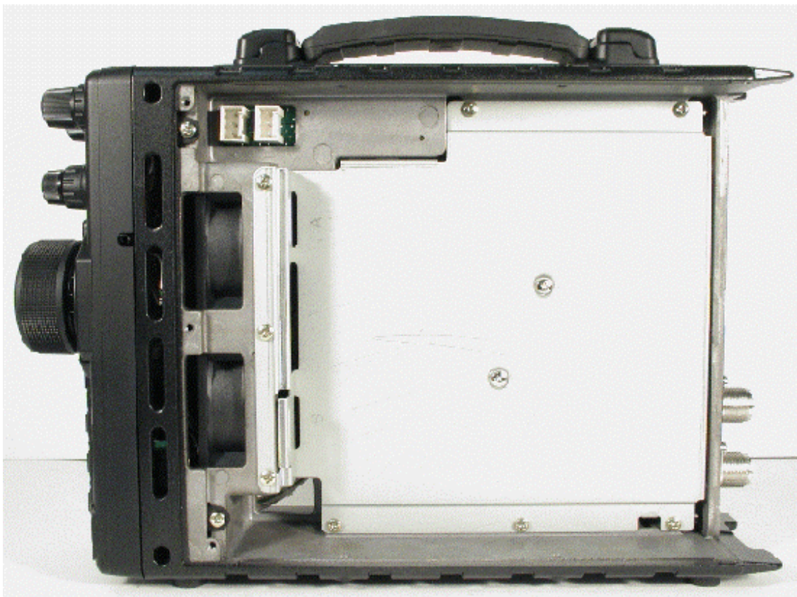
Open Bottom Case
