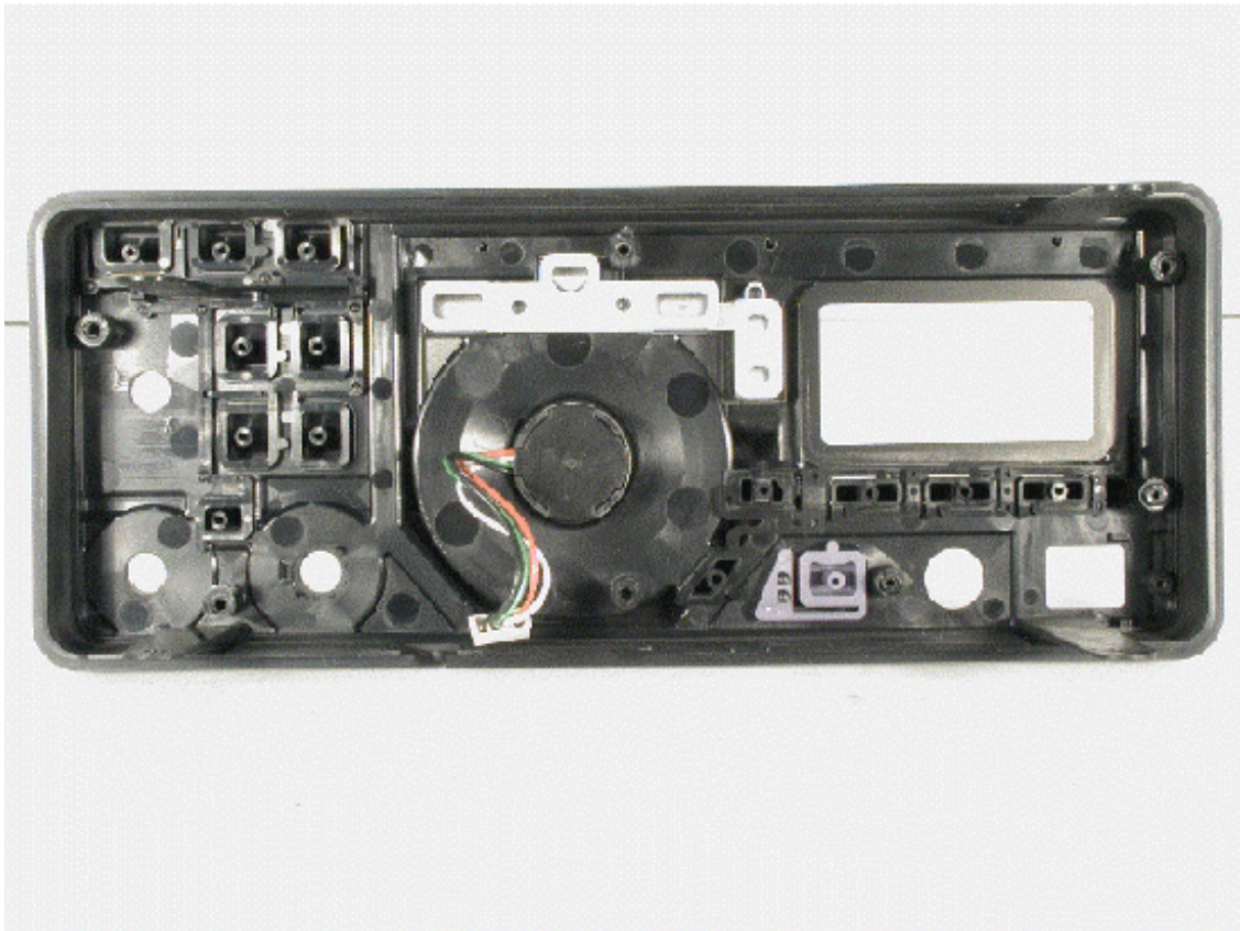
Inside Top of Chassis
