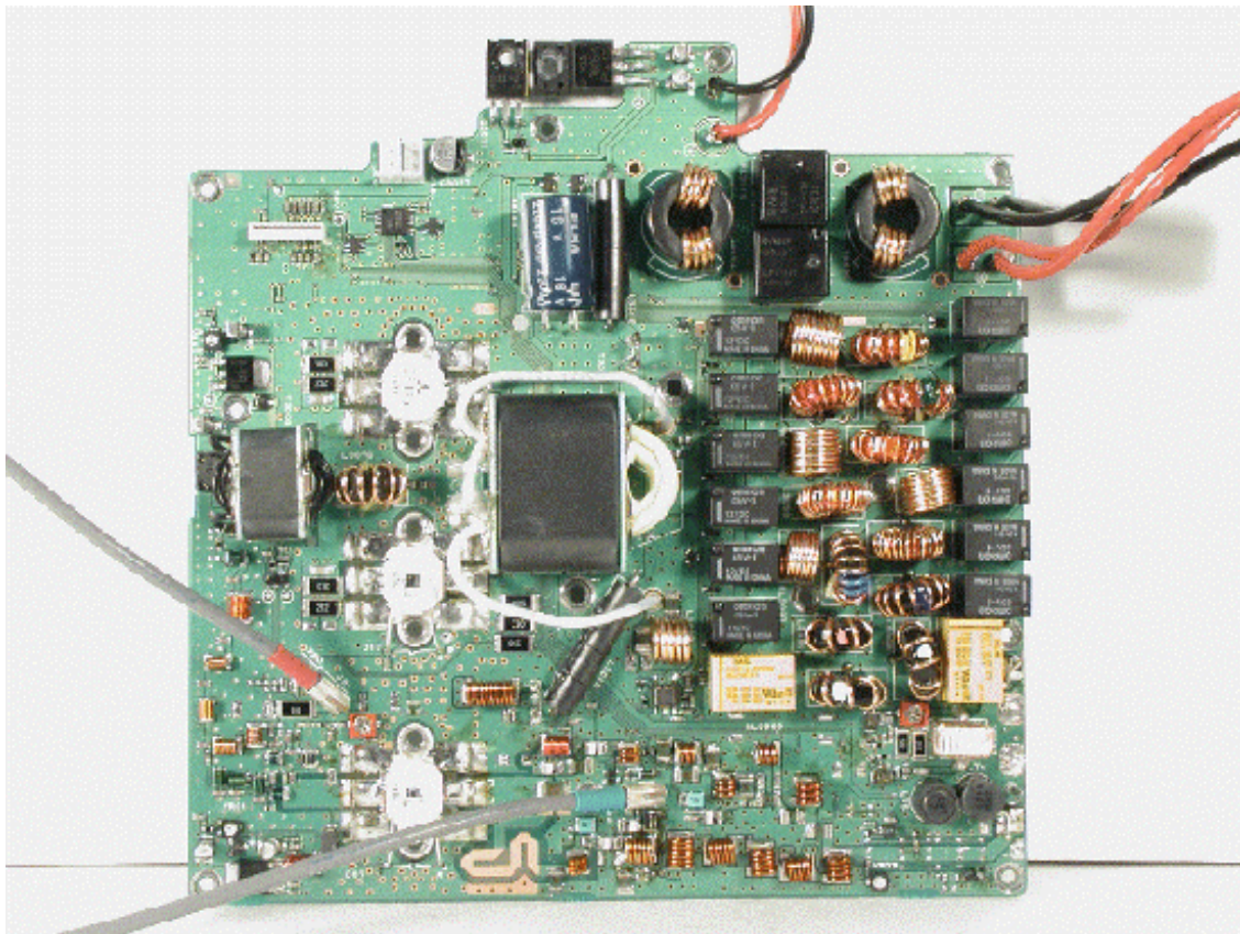
Side-A of PA-UNIT
