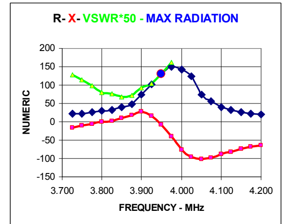
FIGURE 11 – BEFORE ADDING THE SOURCE COIL
