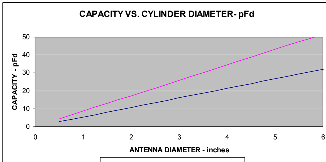
FIGURE 9 - CAPACITY VS
