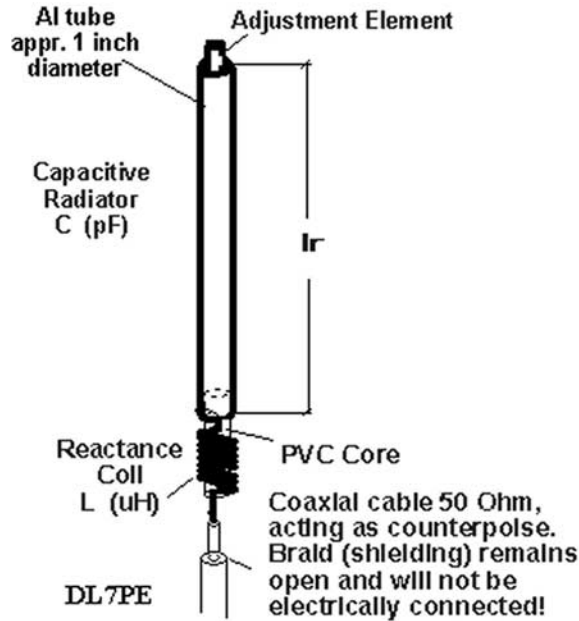
Fig.4 Principle design of a DL7PE-MicroVert Monopole
