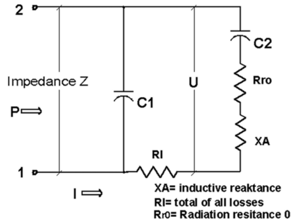
Equivalent Circuit of the DL7PE-MicroVert
