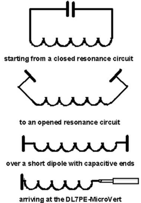
Fig.1: Evolution from a closed resonance circuit to the open series L/C circuit of the DL7PE-MicroVert
