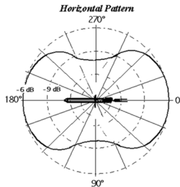
Fig. 8 Horizontal-Plane Radiation Pattern of the DL7PE-MicroVert
