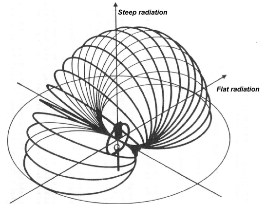
Fig. 7 Radiation pattern of a vertical small magnetic Loop more or less identical with that of the DL7PE-MicroVert
