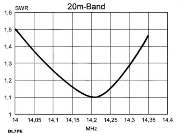
Fig.6: Typical SWR-diagram for the 20m band
