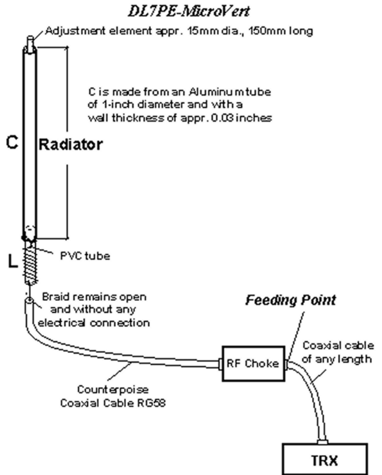
Fig. 5 Choke according To W1JR
