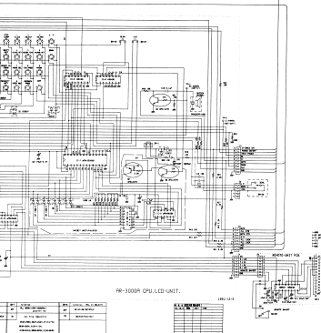
CPU/LCD UNIT
