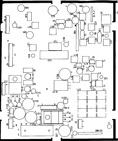
MAIN UNIT PARTS LAYOUT
