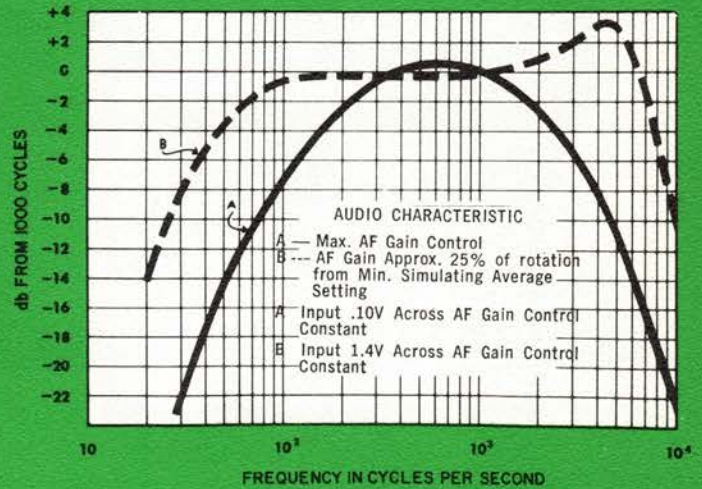
AUTO-RESPONSE CURVE
