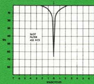
SLOT FILTER
