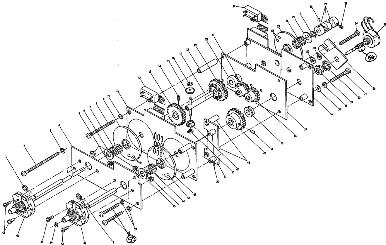
Figure 8D-7. A9 Peak Deviation and Range Switch Assembly Illustrated Parts Breakdown
